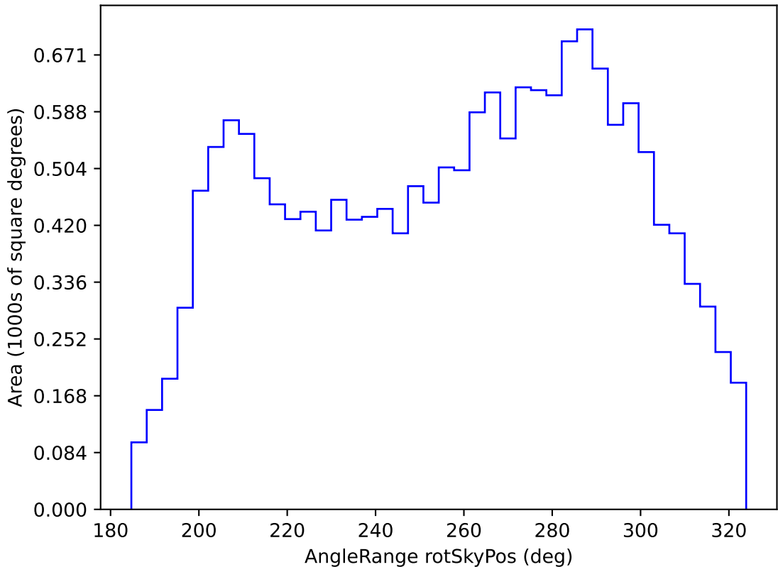
too_elab_r8_d3_griz_v3.4_10yrs WFD u band: AngleRange rotSkyPos
