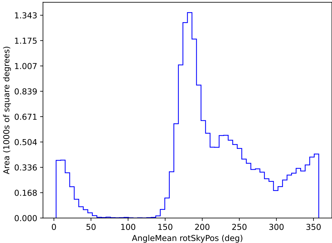
too_elab_r8_d3_griz_v3.4_10yrs WFD u band: AngleMean rotSkyPos
