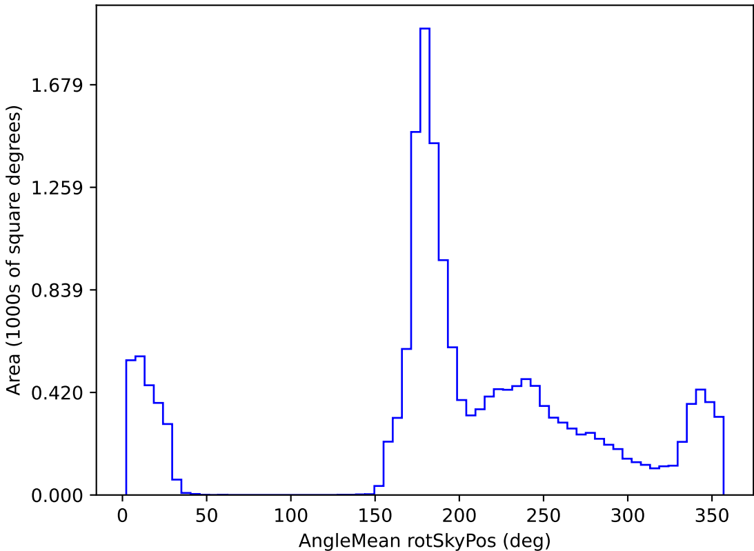
too_elab_r8_d3_griz_v3.4_10yrs WFD r band: AngleMean rotSkyPos
