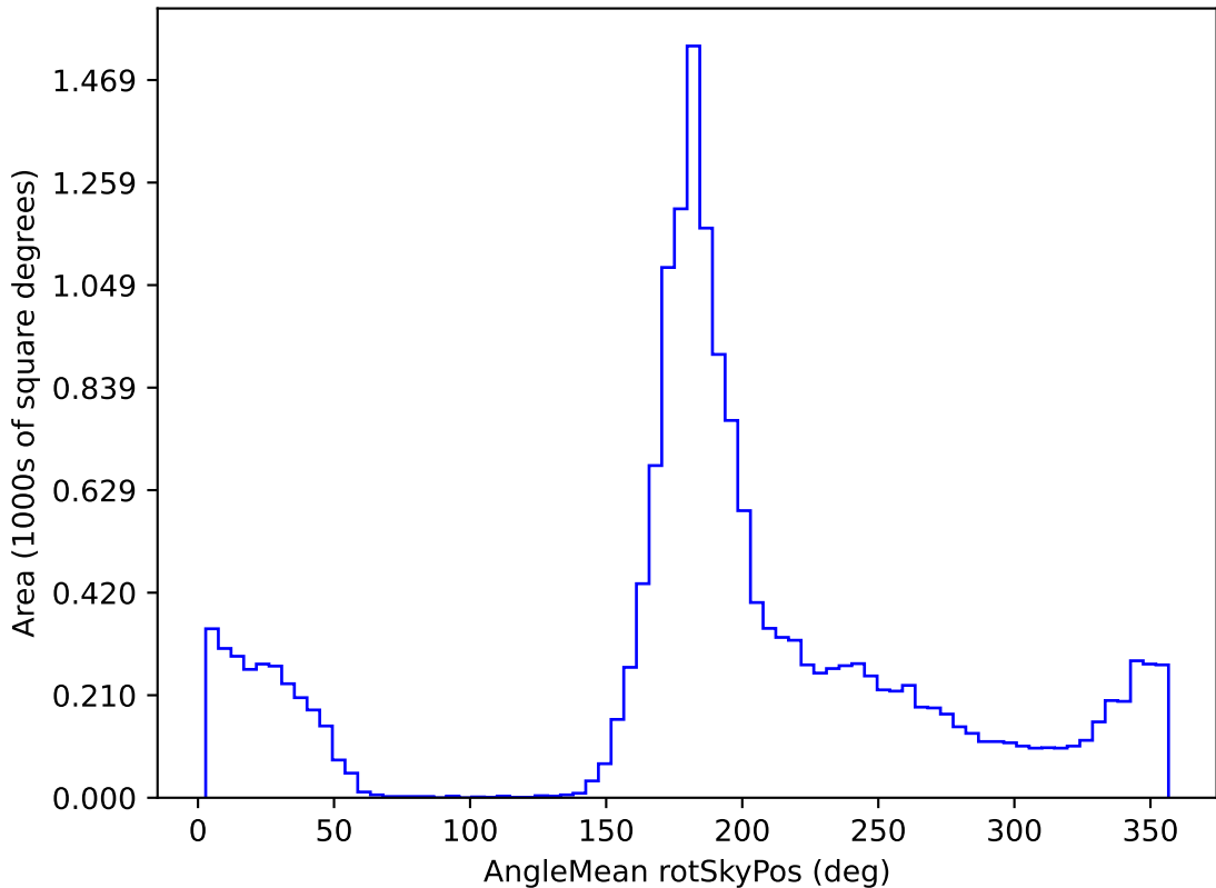
too_elab_r8_d3_griz_v3.4_10yrs WFD g band: AngleMean rotSkyPos
