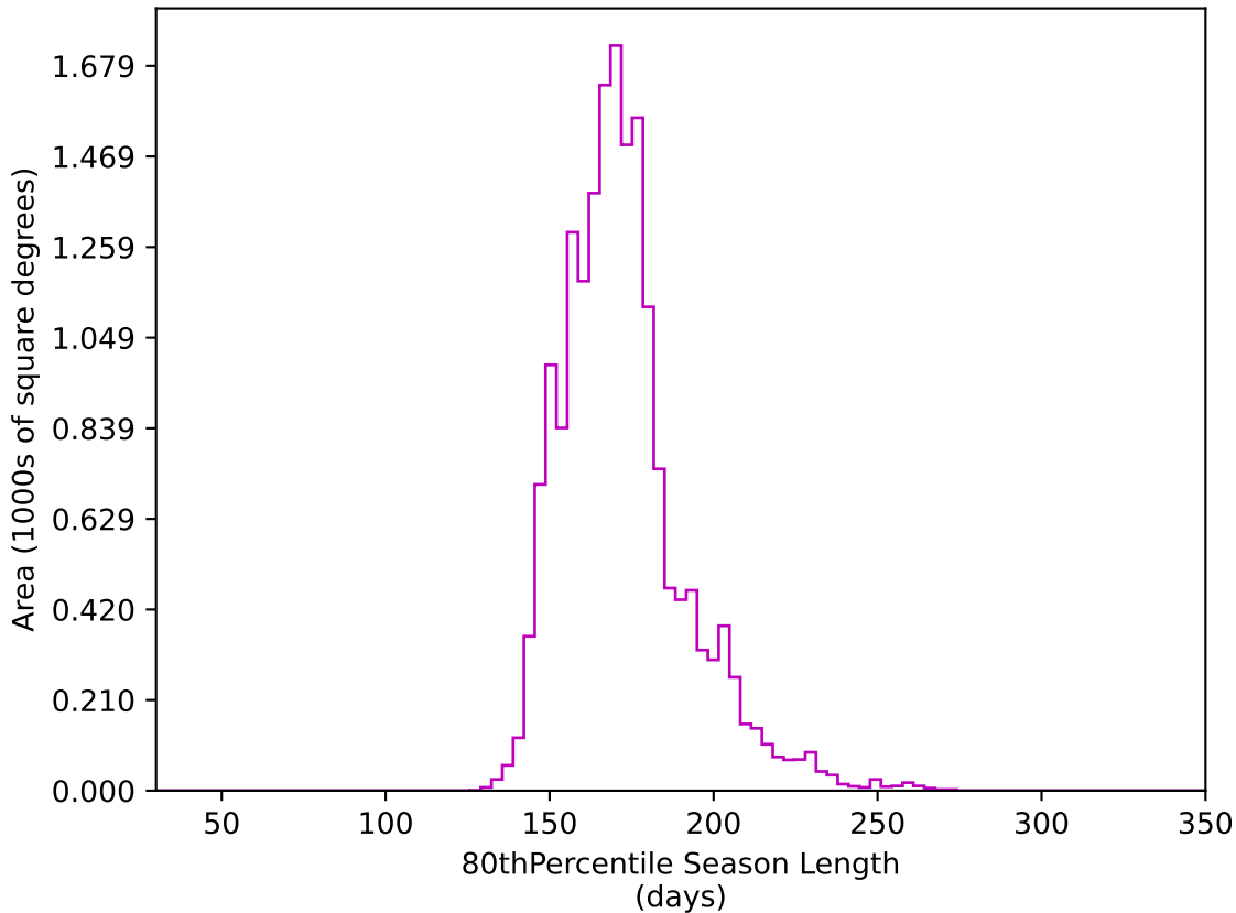
too_elab_r8_d3_griz_v3.4_10yrs WFD z band: 80thPercentile Season Length
