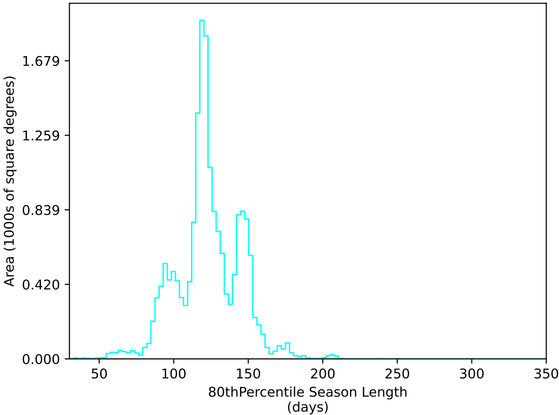
too_elab_r8_d3_griz_v3.4_10yrs WFD u band: 80thPercentile Season Length
