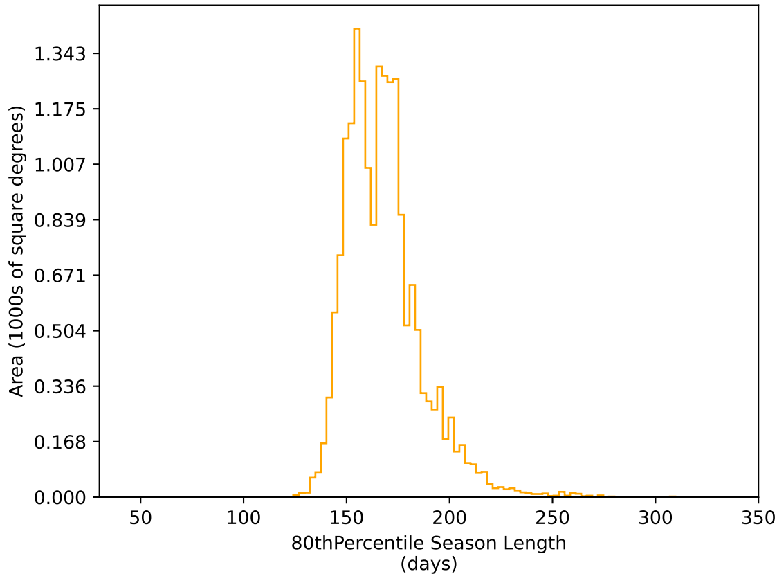
too_elab_r8_d3_griz_v3.4_10yrs WFD r band: 80thPercentile Season Length
