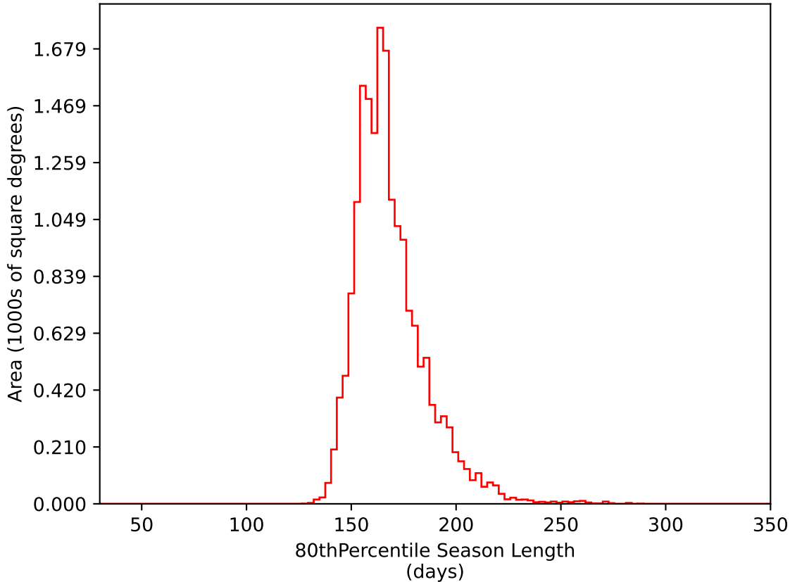
too_elab_r8_d3_griz_v3.4_10yrs WFD i band: 80thPercentile Season Length
