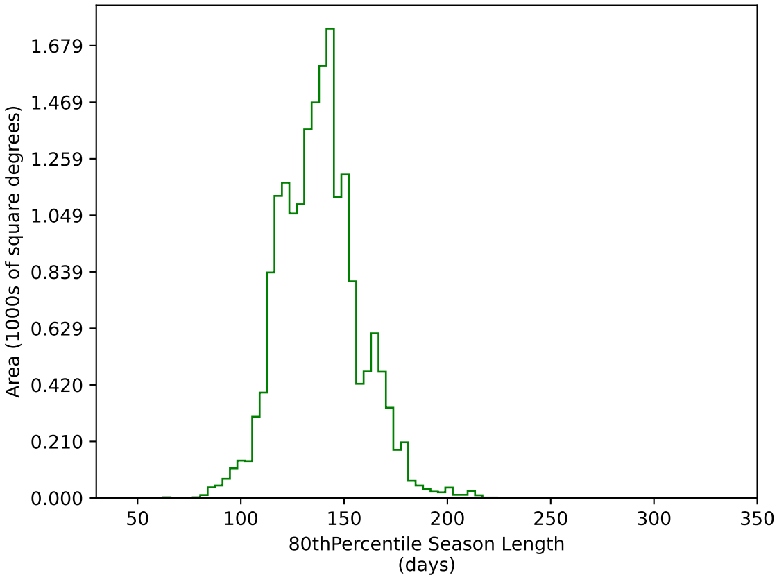
too_elab_r8_d3_griz_v3.4_10yrs WFD g band: 80thPercentile Season Length
