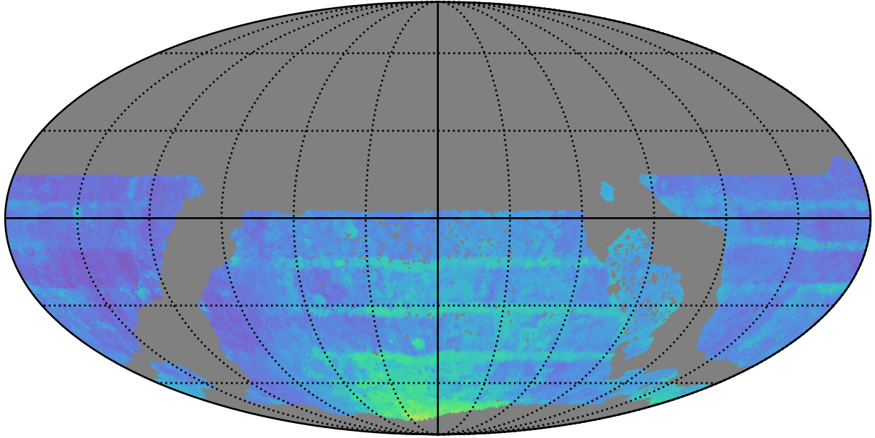
too_elab_r8_d3_griz_v3.4_10yrs WFD all bands: 80thPercentile Season Length
