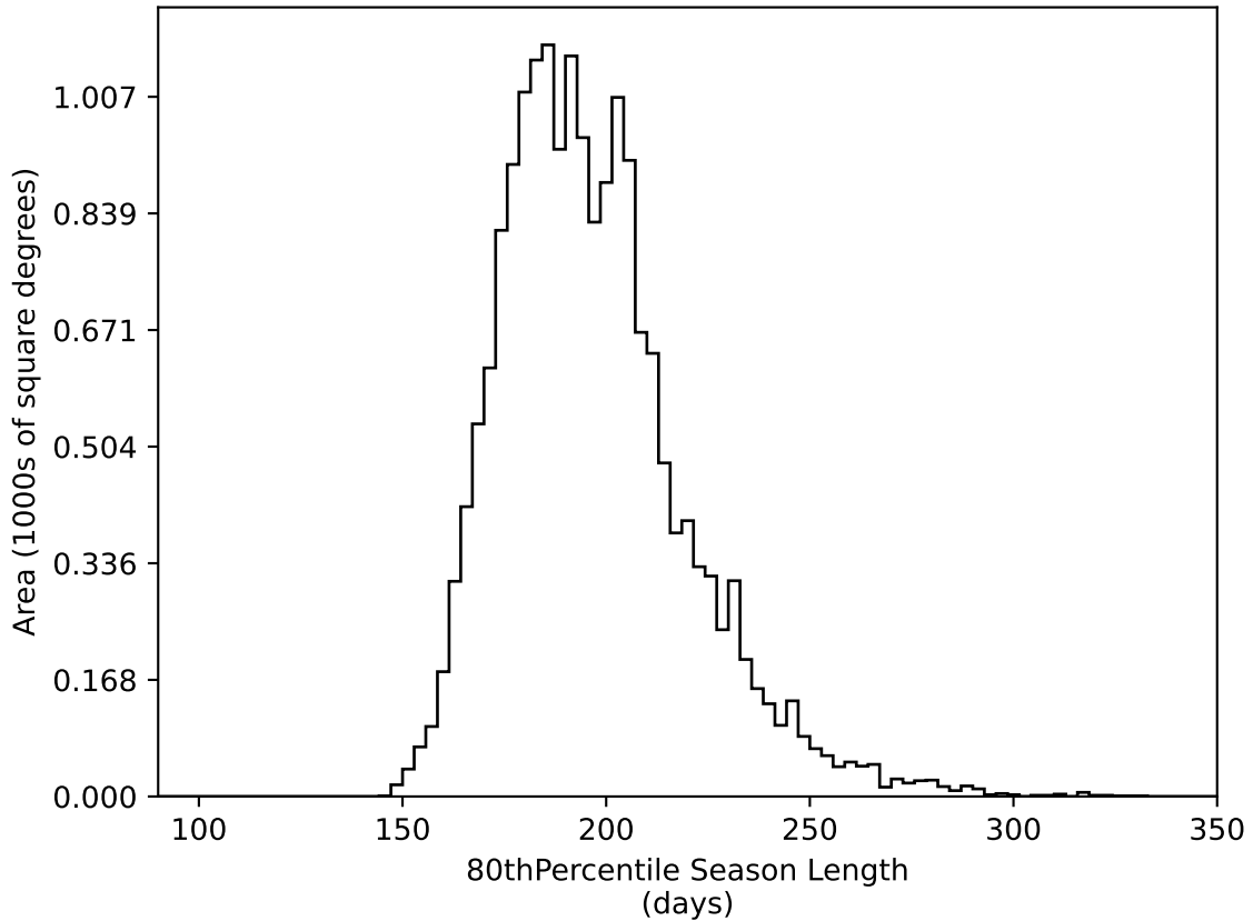
too_elab_r8_d3_griz_v3.4_10yrs WFD all bands: 80thPercentile Season Length
