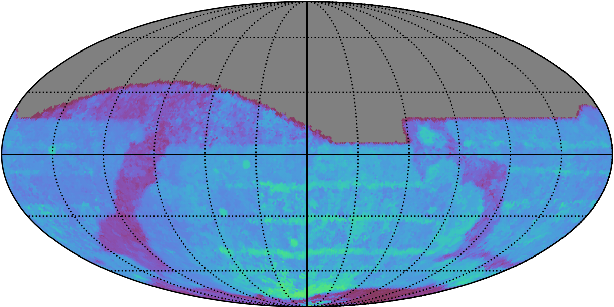
too_elab_r8_d3_griz_v3.4_10yrs All sky z band: 80thPercentile Season Length
