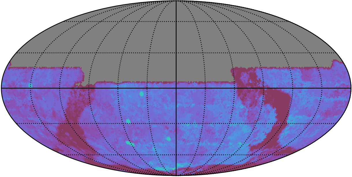
too_elab_r8_d3_griz_v3.4_10yrs All sky u band: 80thPercentile Season Length
