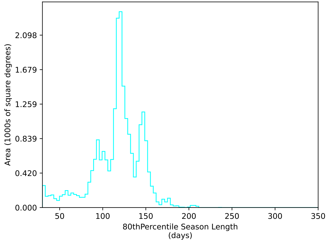
too_elab_r8_d3_griz_v3.4_10yrs All sky u band: 80thPercentile Season Length
