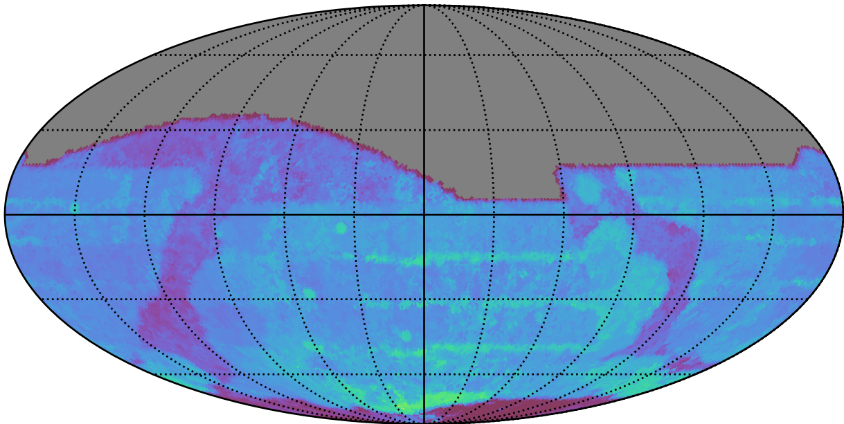
too_elab_r8_d3_griz_v3.4_10yrs All sky r band: 80thPercentile Season Length
