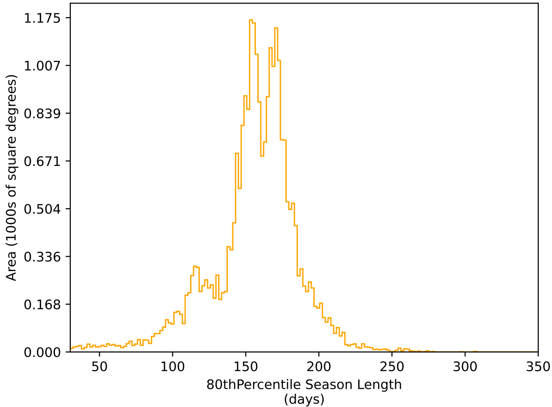
too_elab_r8_d3_griz_v3.4_10yrs All sky r band: 80thPercentile Season Length
