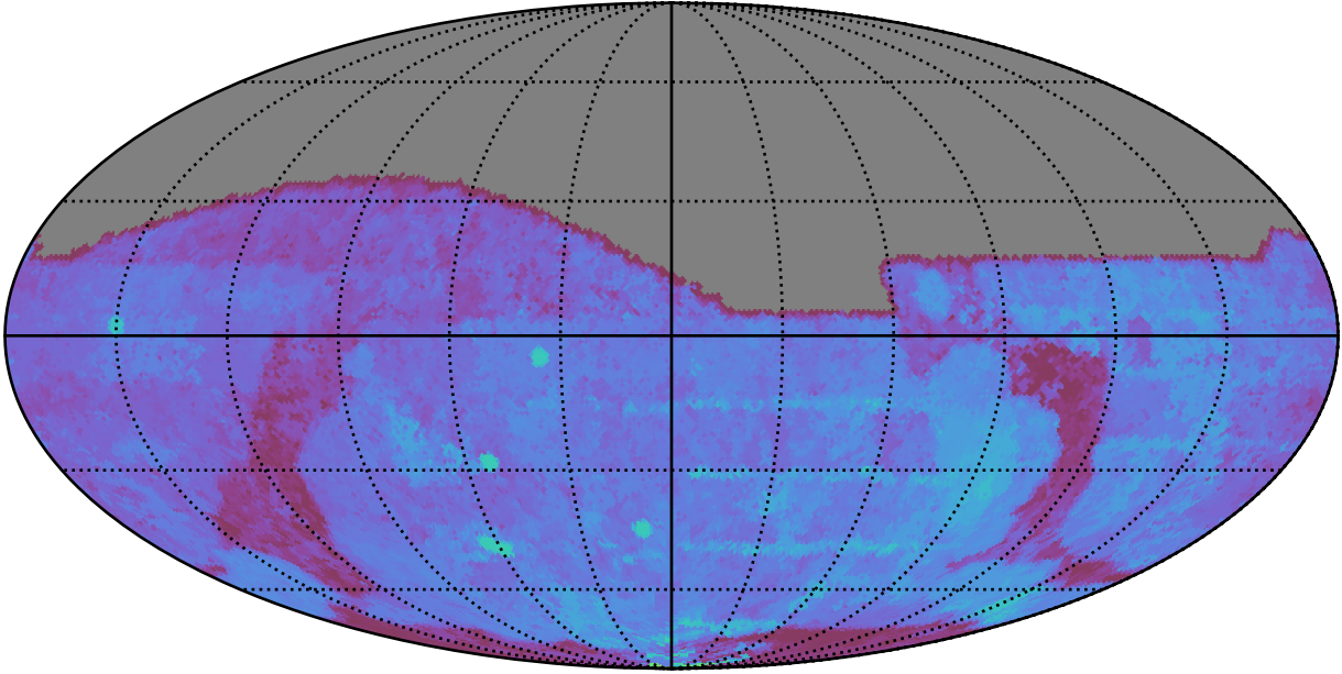
too_elab_r8_d3_griz_v3.4_10yrs All sky g band: 80thPercentile Season Length
