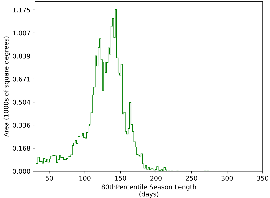
too_elab_r8_d3_griz_v3.4_10yrs All sky g band: 80thPercentile Season Length
