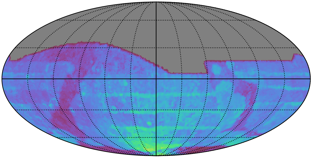
too_elab_r8_d3_griz_v3.4_10yrs All sky all bands: 80thPercentile Season Length
