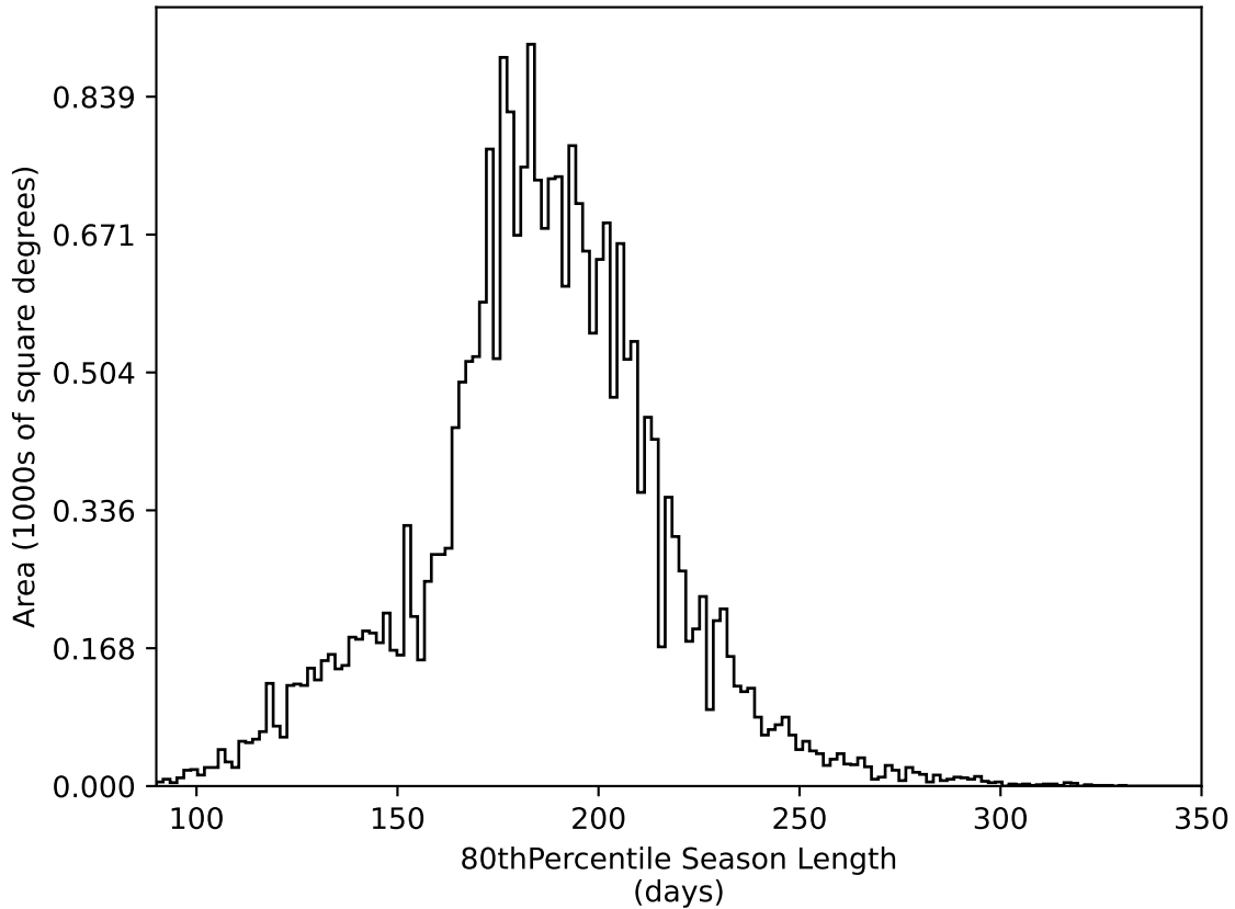
too_elab_r8_d3_griz_v3.4_10yrs All sky all bands: 80thPercentile Season Length
