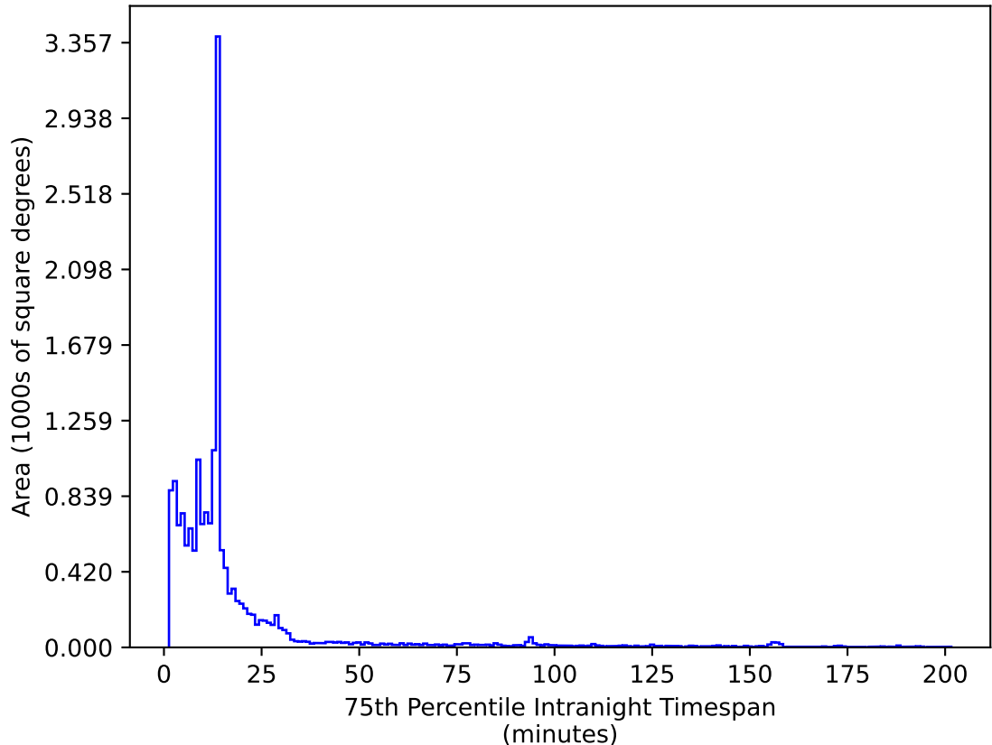
too_elab_r8_d3_griz_v3.4_10yrs WFD z band: 75th Percentile Intranight Timespan
