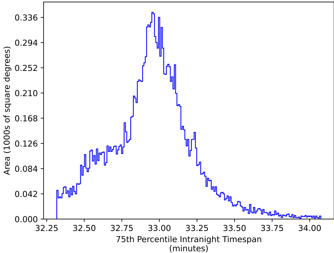
too_elab_r8_d3_griz_v3.4_10yrs WFD y band: 75th Percentile Intranight Timespan
