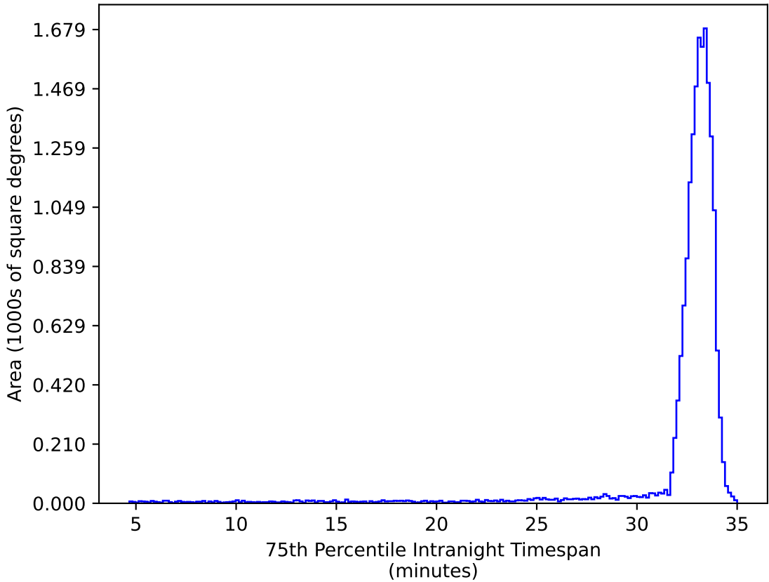
too_elab_r8_d3_griz_v3.4_10yrs WFD ug bands: 75th Percentile Intranight Timespan
