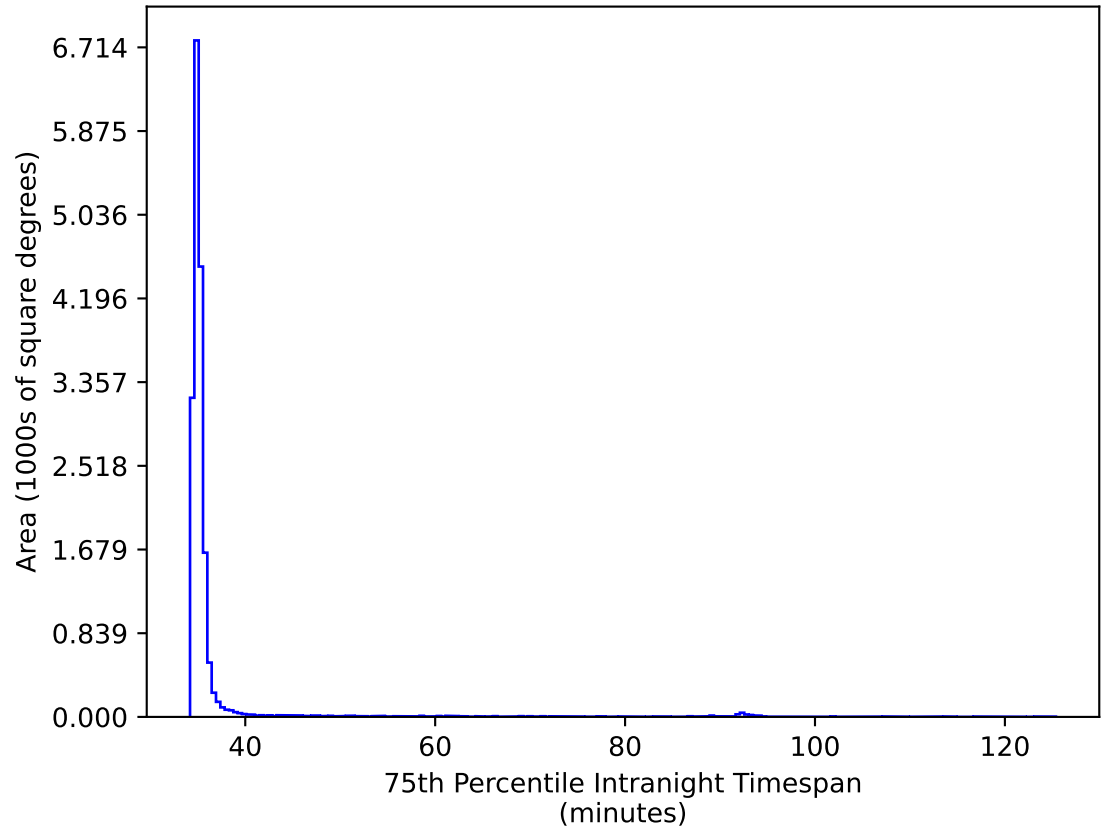
too_elab_r8_d3_griz_v3.4_10yrs WFD ri bands: 75th Percentile Intranight Timespan
