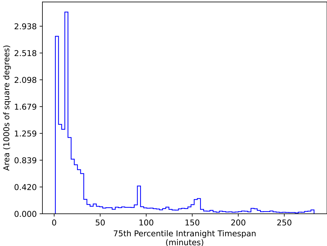
too_elab_r8_d3_griz_v3.4_10yrs WFD r band: 75th Percentile Intranight Timespan
