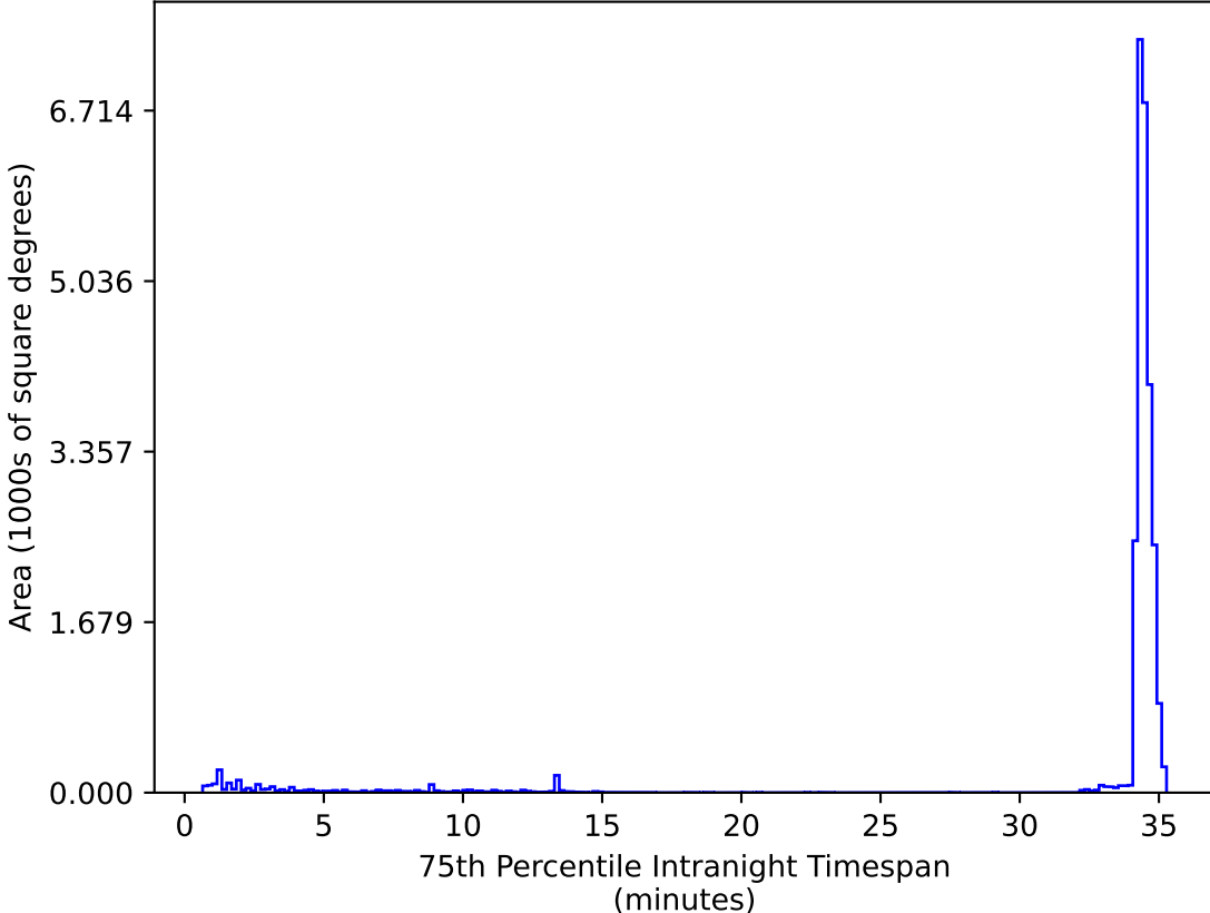
too_elab_r8_d3_griz_v3.4_10yrs All sky zy bands: 75th Percentile Intranight Timespan
