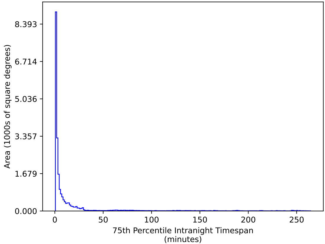
too_elab_r8_d3_griz_v3.4_10yrs All sky u band: 75th Percentile Intranight Timespan
