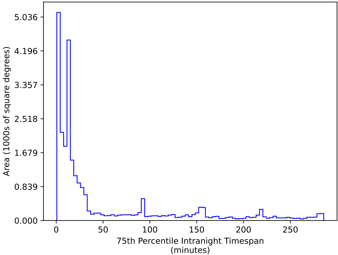
too_elab_r8_d3_griz_v3.4_10yrs All sky r band: 75th Percentile Intranight Timespan
