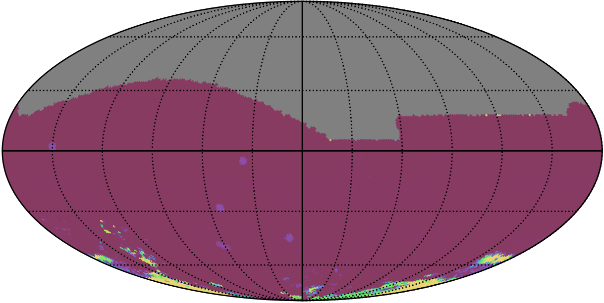
too_elab_r8_d3_griz_v3.4_10yrs All sky iz bands: 75th Percentile Intranight Timespan
