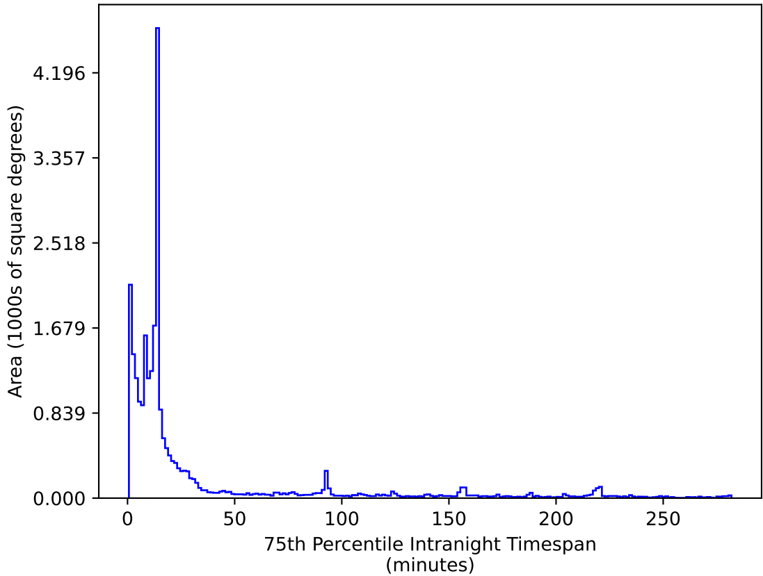
too_elab_r8_d3_griz_v3.4_10yrs All sky i band: 75th Percentile Intranight Timespan
