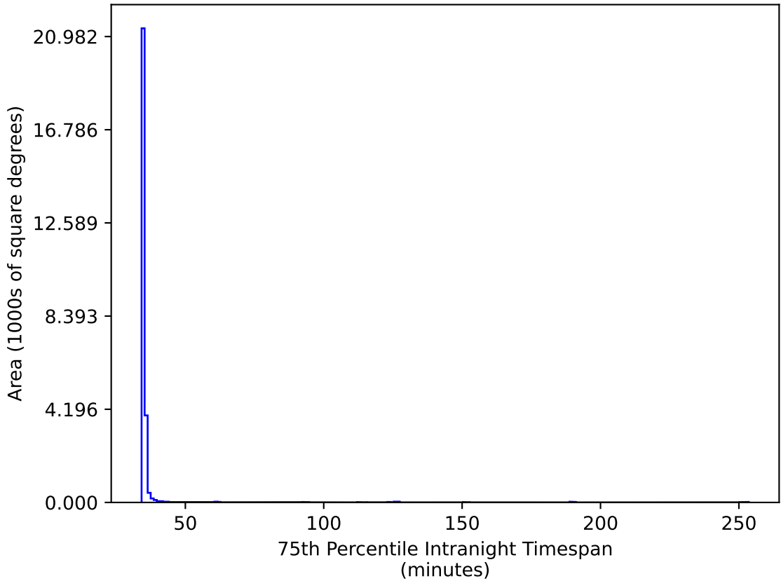
too_elab_r8_d3_griz_v3.4_10yrs All sky gr bands: 75th Percentile Intranight Timespan
