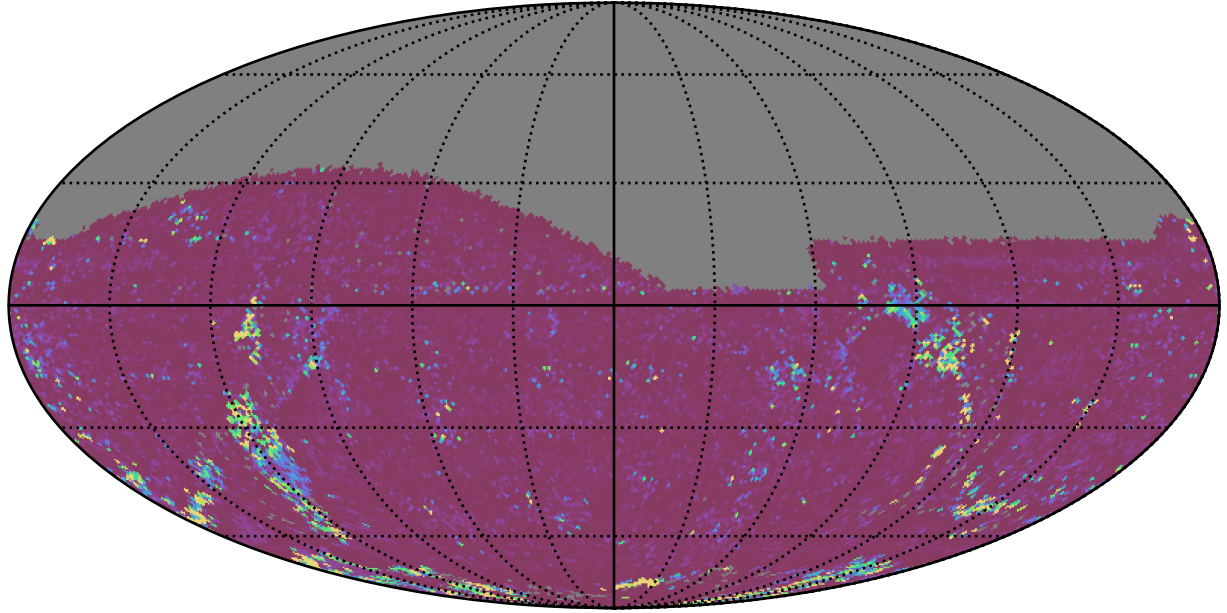
too_elab_r8_d3_griz_v3.4_10yrs All sky g band: 75th Percentile Intranight Timespan
