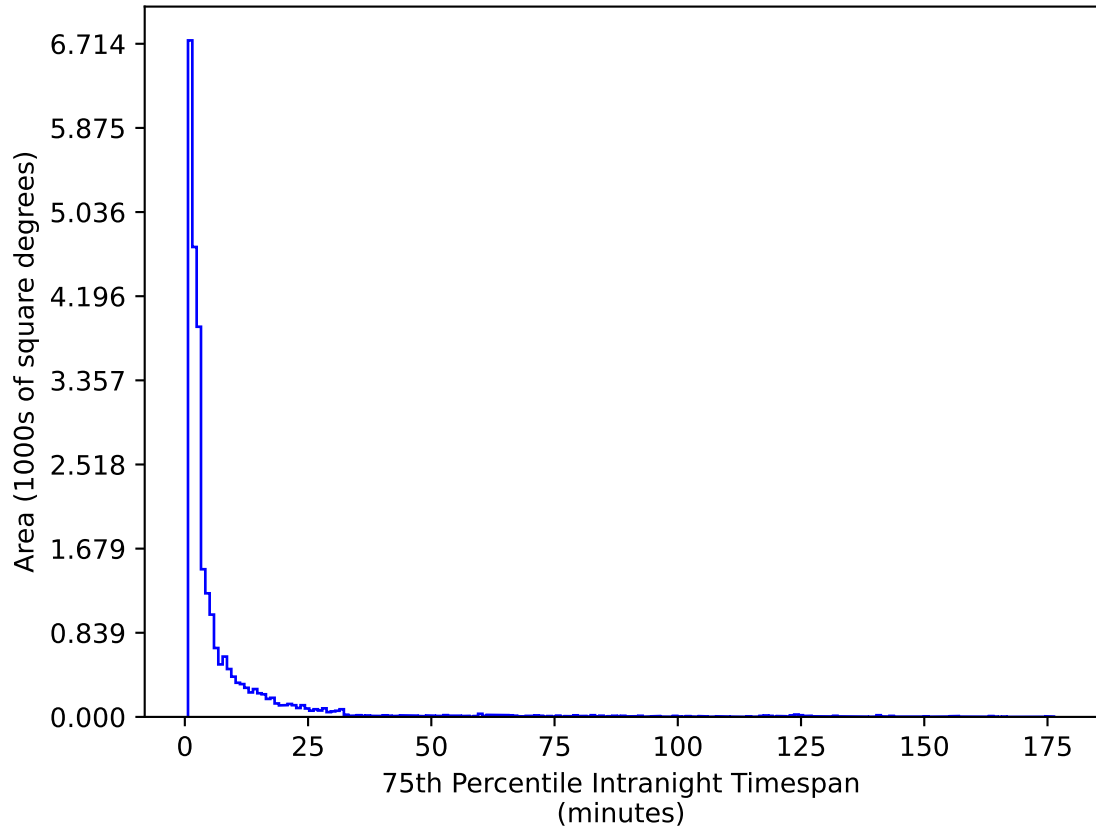
too_elab_r8_d3_griz_v3.4_10yrs All sky g band: 75th Percentile Intranight Timespan
