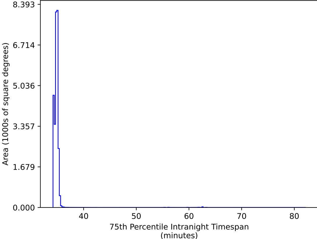
too_elab_r8_d3_griz_v3.4_10yrs All sky all bands: 75th Percentile Intranight Timespan
