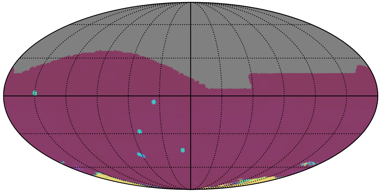
too_elab_r8_d3_griz_v3.4_10yrs All sky: 75th Percentile Intranight Timespan
