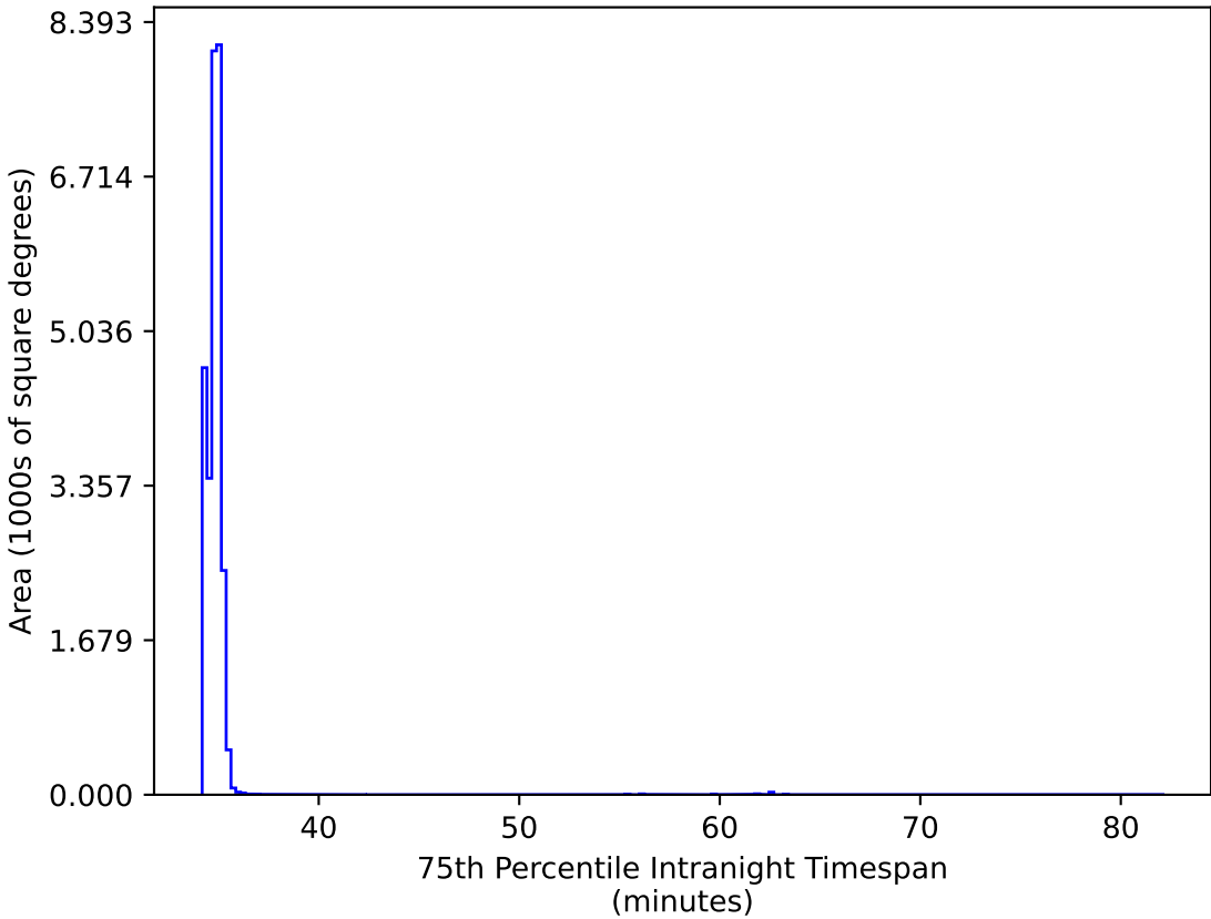
too_elab_r8_d3_griz_v3.4_10yrs All sky: 75th Percentile Intranight Timespan
