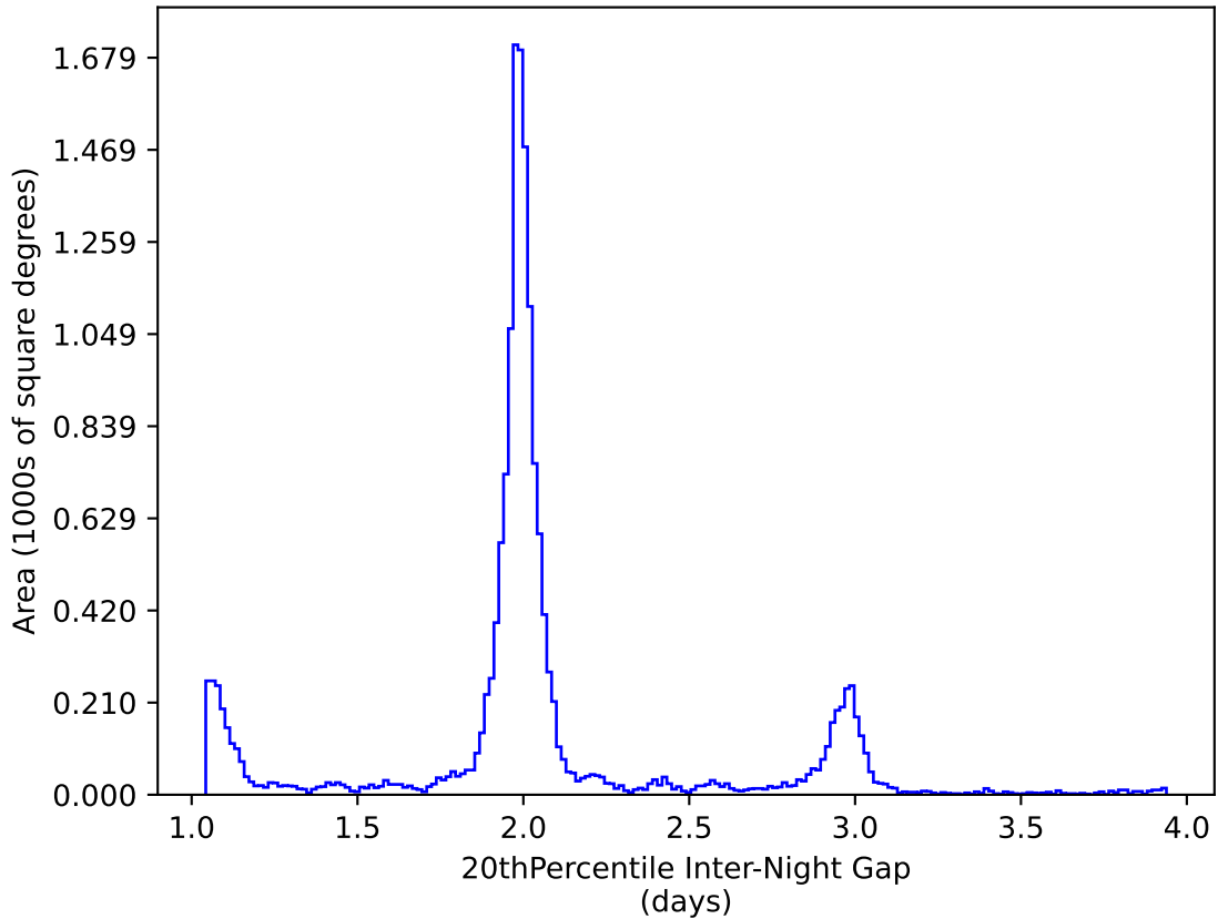
too_elab_r8_d3_griz_v3.4_10yrs WFD y band: 20thPercentile Inter-Night Gap
