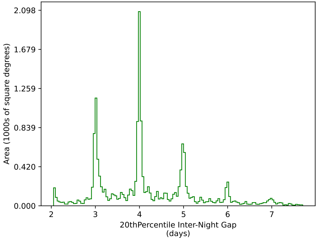
too_elab_r8_d3_griz_v3.4_10yrs WFD g band: 20thPercentile Inter-Night Gap
