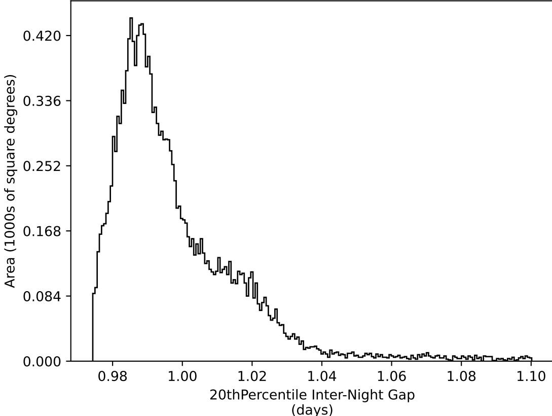
too_elab_r8_d3_griz_v3.4_10yrs WFD all bands: 20thPercentile Inter-Night Gap
