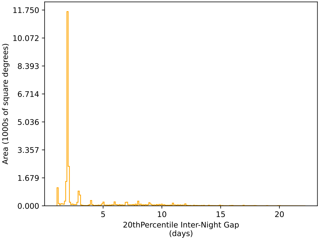
too_elab_r8_d3_griz_v3.4_10yrs All sky r band: 20thPercentile Inter-Night Gap
