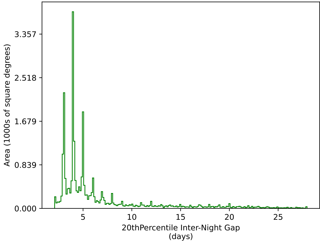
too_elab_r8_d3_griz_v3.4_10yrs All sky g band: 20thPercentile Inter-Night Gap
