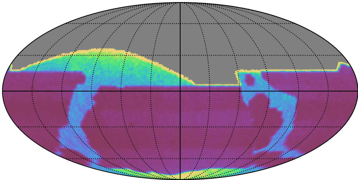
too_elab_r8_d3_griz_v3.4_10yrs : properMotion
