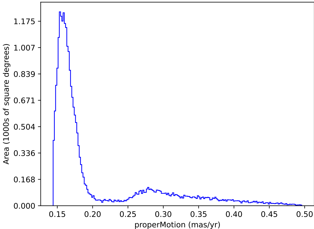
too_elab_r8_d3_griz_v3.4_10yrs : properMotion
