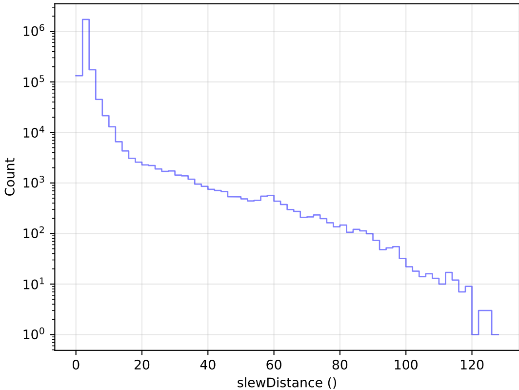
too_elab_r8_d3_griz_v3.4_10yrs All visits: Slew Distance Histogram
