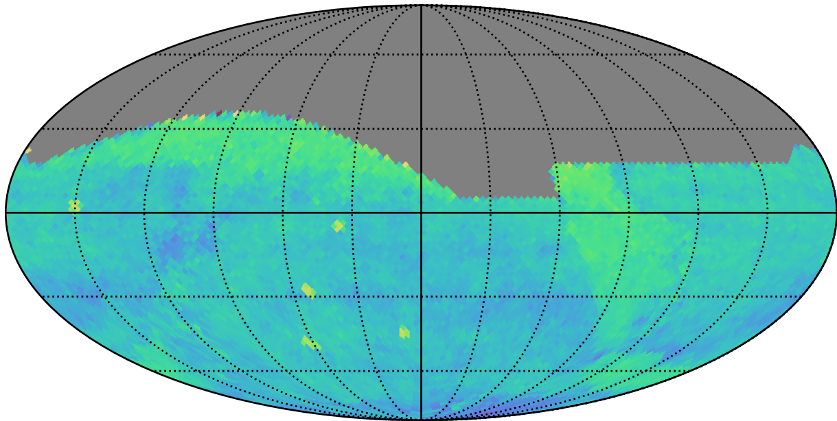
too_elab_r8_d3_griz_v3.4_10yrs (g or r or i): PairFraction
