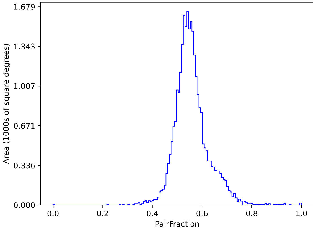
too_elab_r8_d3_griz_v3.4_10yrs (g or r or i): PairFraction
