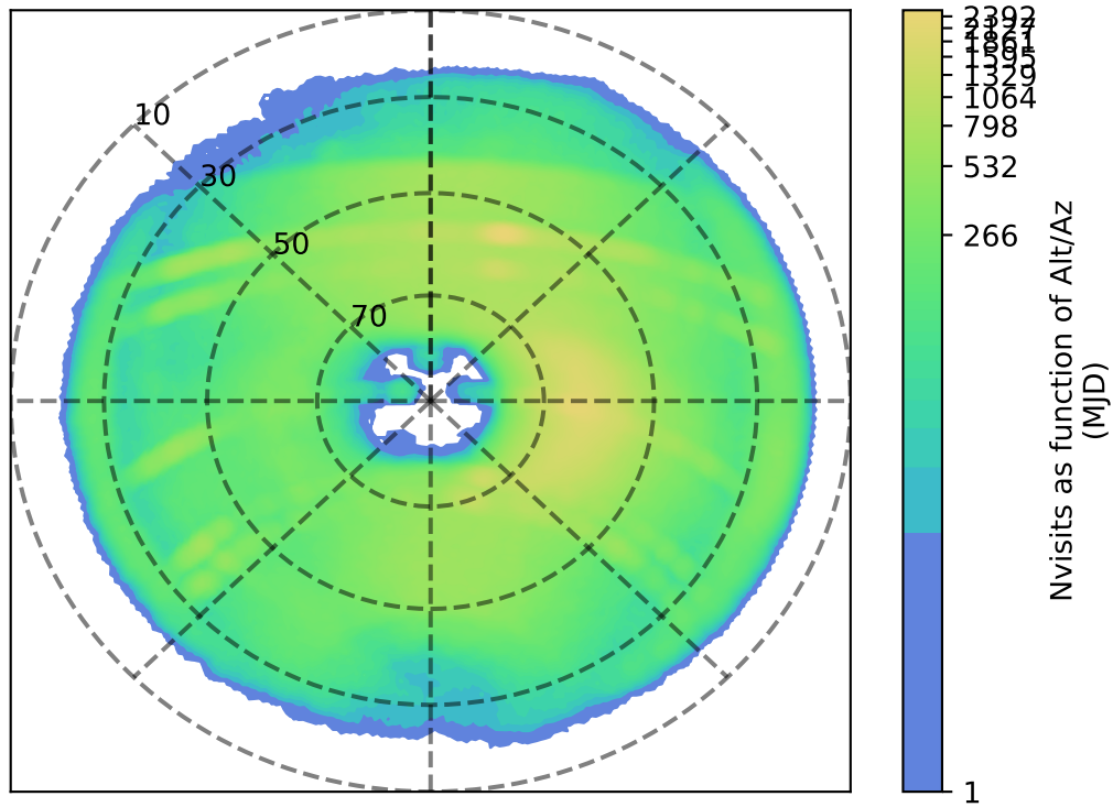
too_elab_r8_d3_griz_v3.4_10yrs z: Nvisits as function of Alt/Az
