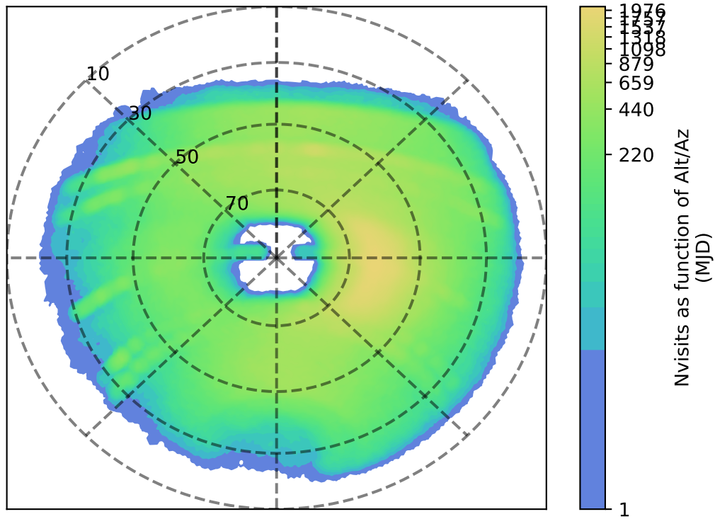
too_elab_r8_d3_griz_v3.4_10yrs y: Nvisits as function of Alt/Az
