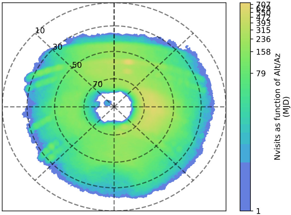
too_elab_r8_d3_griz_v3.4_10yrs u: Nvisits as function of Alt/Az
