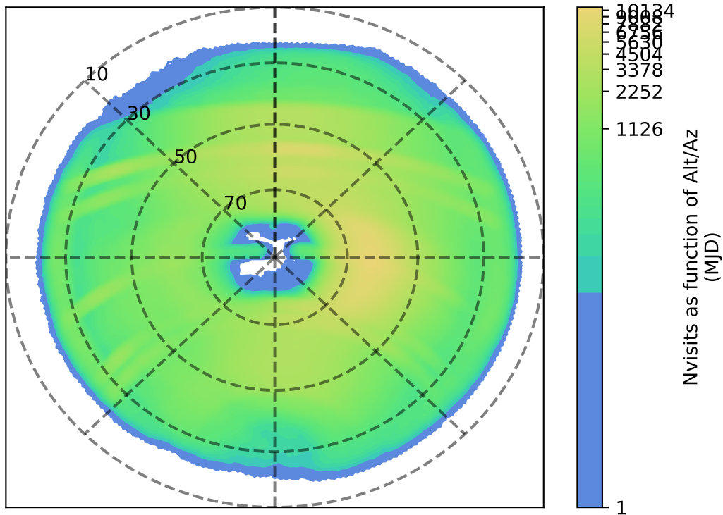
too_elab_r8_d3_griz_v3.4_10yrs : Nvisits as function of Alt/Az
